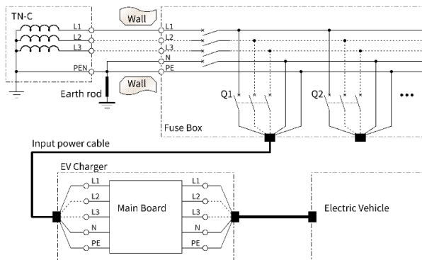
Fig. 5-4 HM10 work in TN-C system with earth rod
