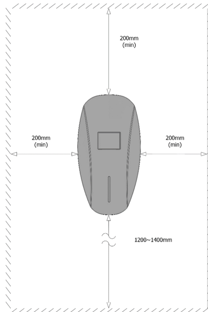
Fig. 5-2 Minimum space requirements for wall mounting
