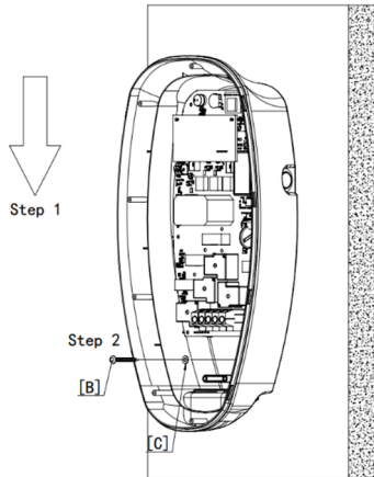
Fig. 5-8 Install the Wall Box
