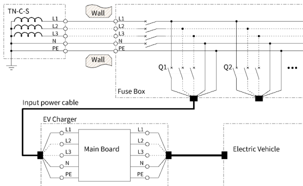
Fig. 5-3 HM10 work in TN-S system
