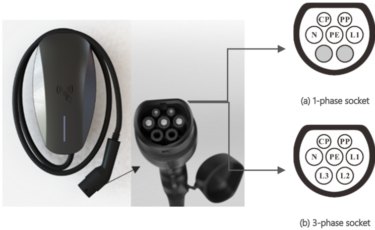
Fig. 3-3 Schematic diagram of Type 2 socket on M3B series products
