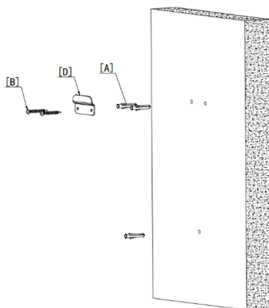
Fig. 5-6 Fixed the Wall-mounting accessories-D
