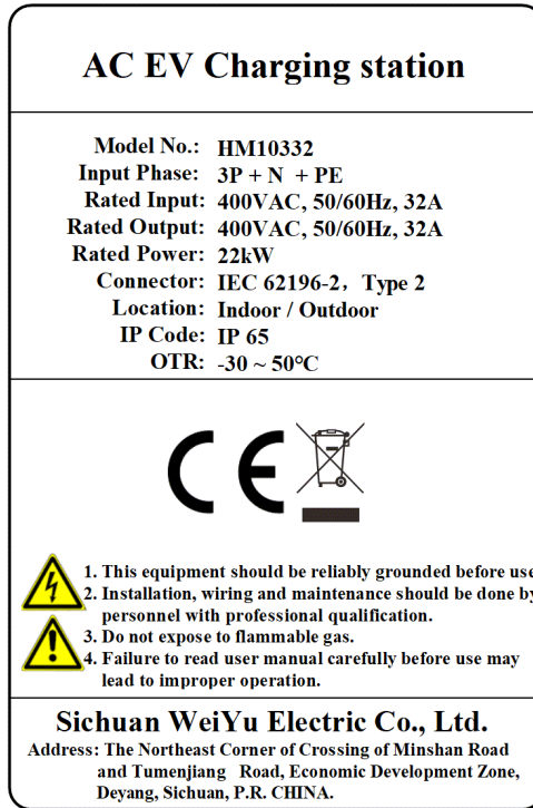
Fig. 4-4 The location and content of the nameplate
